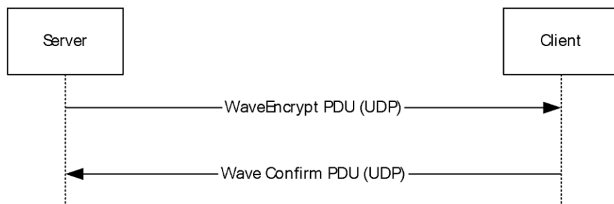
Figure 5: Data transfer sequence over UDP
